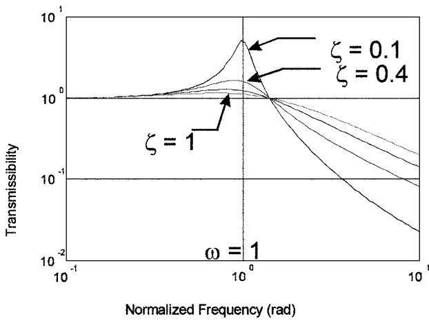
Fig. 4 Transmissibility of second-order system.
