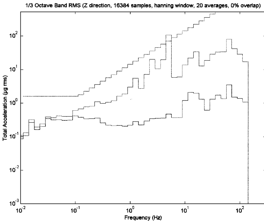
Fig. 8 Comparison of STABLE acceleration (bottom), shuttle acceleration (middle), and station requirement (top) \frac{1}{3} -octave band measurements during crew exercise.
