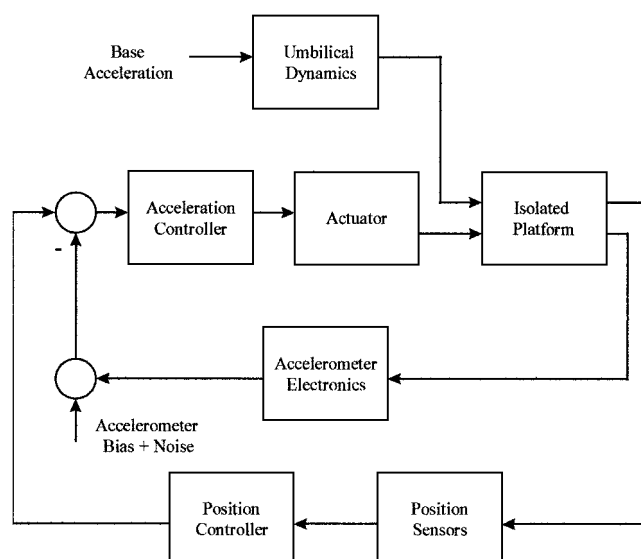
Fig. 6 STABLE general block diagram.
